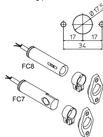
Drilling plane FC7 FC8
