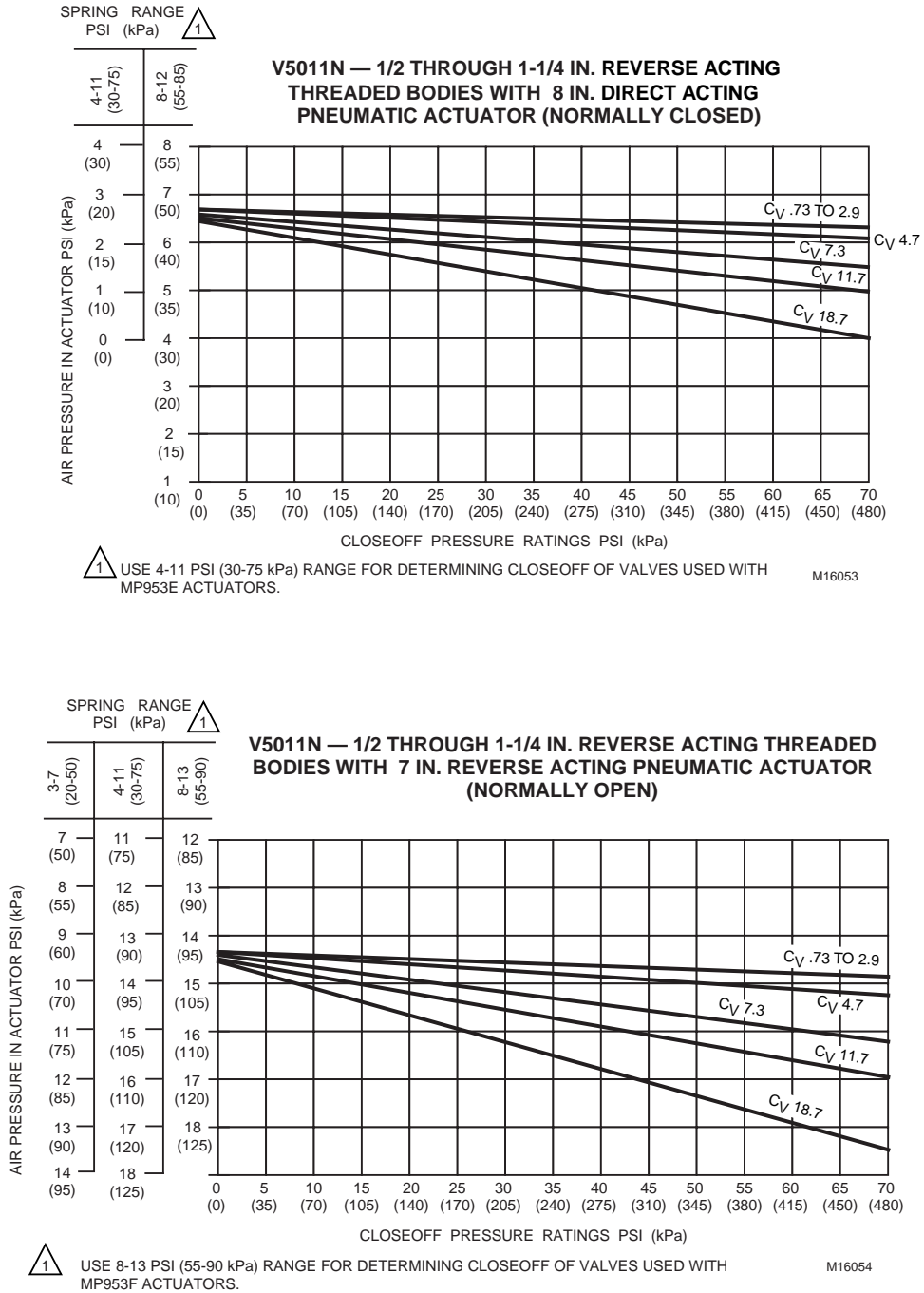
Fig. 2. Close-off pressures at various control air pressures for V5011N Valves and MP953 Pneumatic Actuators (continued).
