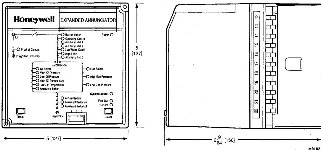
Fig. 2—Mounting dimensions of S7830 Expanded Annunciator and Q7800B Subbase in inches [mm].
