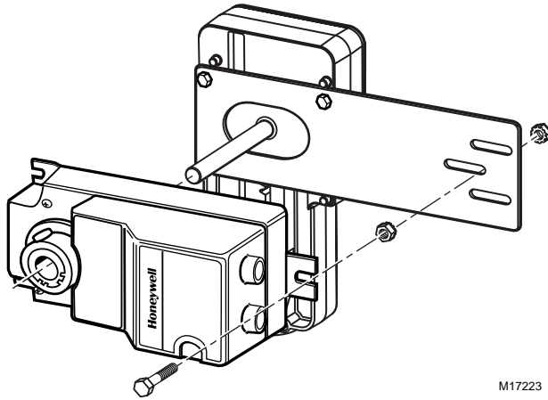
Fig. 5. Installing 150 or 300 lb-in. actuator.
