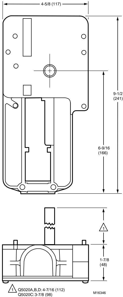
Fig. 1. Q5020 Dimensions in in. (mm).
