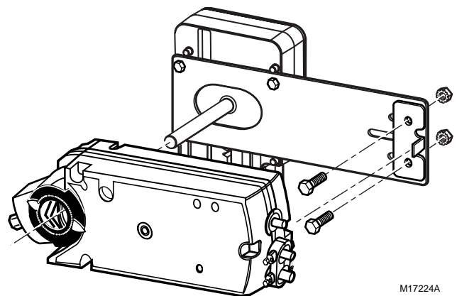
Fig. 4. Installing 142 lb-in. actuator.
