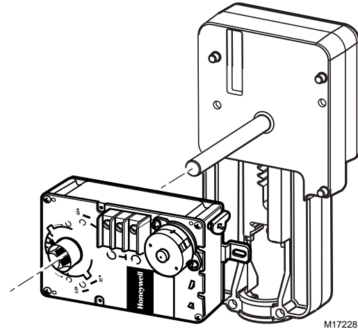
Fig. 6. Installing 35 or 70 lb-in. actuator.
