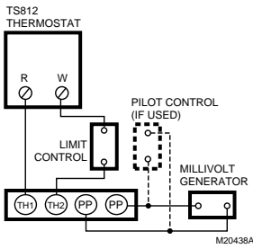
Fig. 5. Typical hookup to TS812A in millivolt system.
