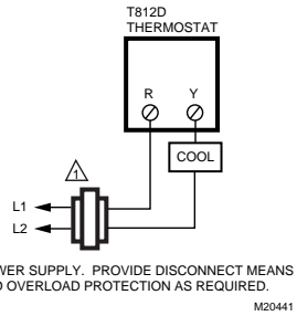
Fig. 8. T812D in cooling only application.
