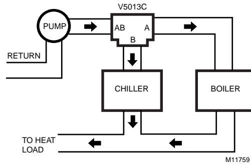
Fig. 6. V5013C diverting valve used to change over complete system.
