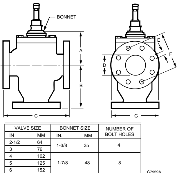
Fig. 1. V5013B,C Flanged Body Dimensions.
